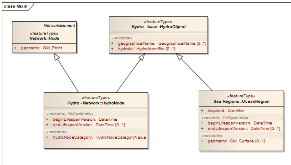
Figure 6 – Mixin example
